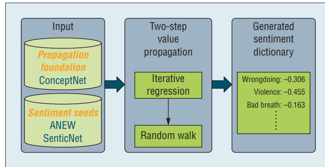
Figure 1. The proposed two-step method. First, iterative regression assigns a sentiment value to ConceptNet's sentiment values. In the second step, these sentiment values are used as starting values for a random-walk method.
