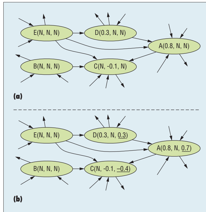
Figure 2. Illustration of value propagation in iterative regression. (a) Concepts A, B, C, D, and E and their Affective Norms for English Words (ANEW), SenticNet, and current value (in parenthesis). (b) Iterative regression step for the concepts.
